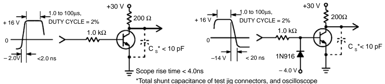
Figure 1. Turn–On Time
